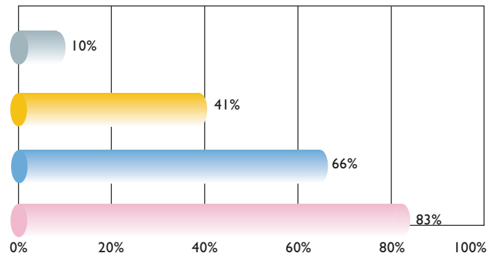
Retention of R-value after repeated exposure to moisture and freeze/thaw conditions Moisture Effects Comparison
